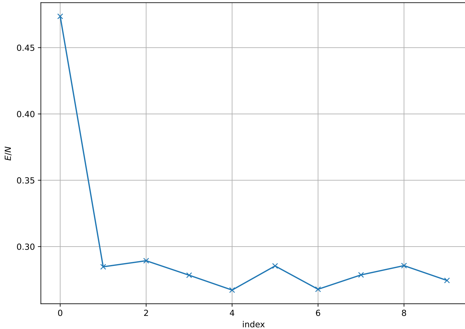
Energy per Site at T = 1.800e - 01 , L = 32
