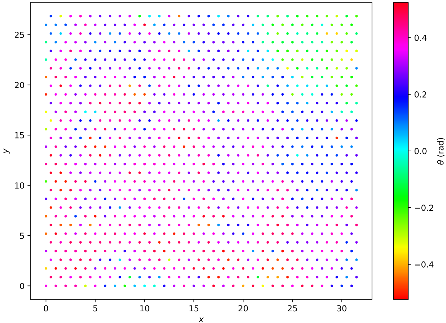
Hexagonal Lattice L=32 , T = 1.80e - 01
