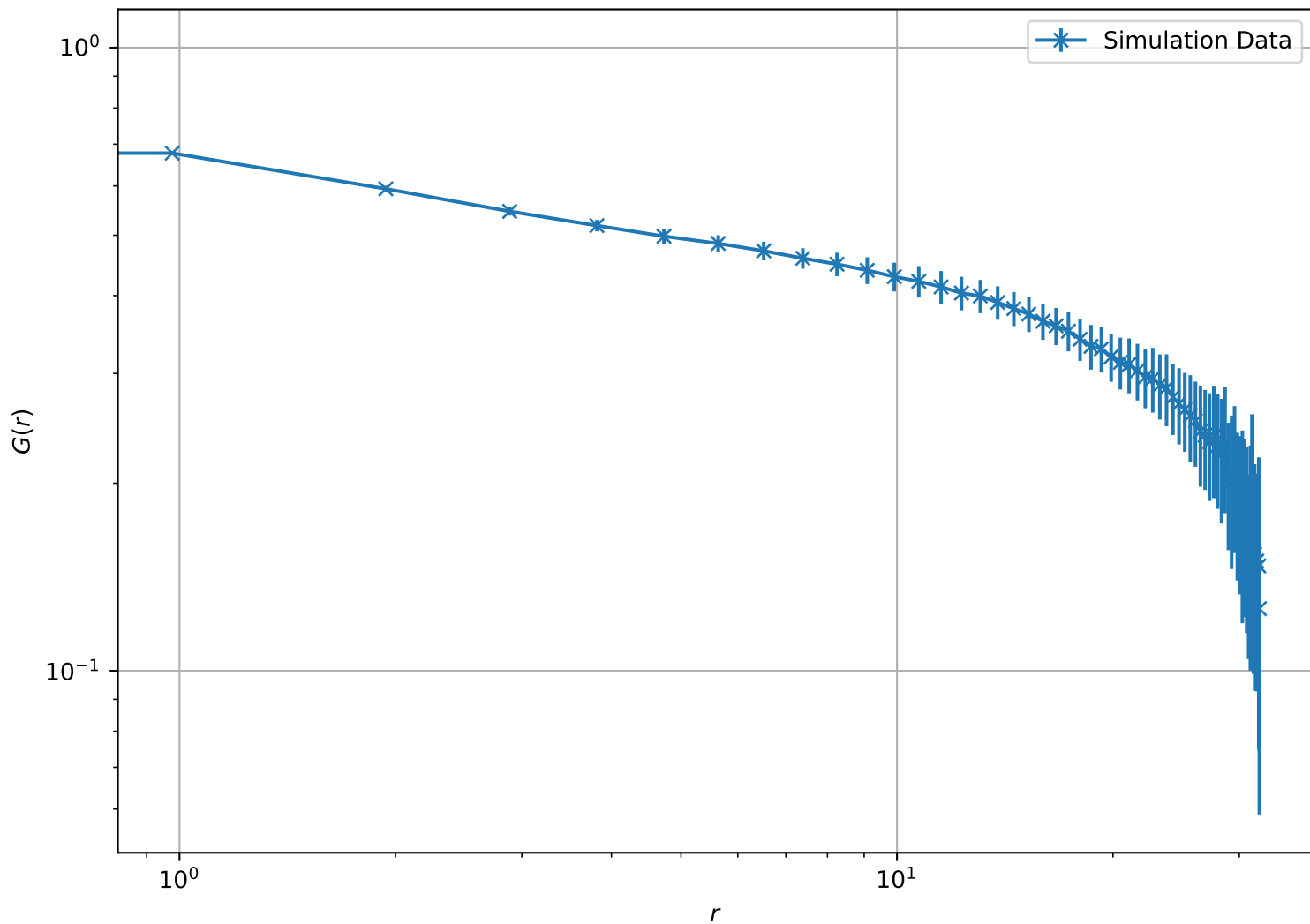
Correlation Function at T = 1.85e - 01 , L = 32 (Log-Log Scale)
