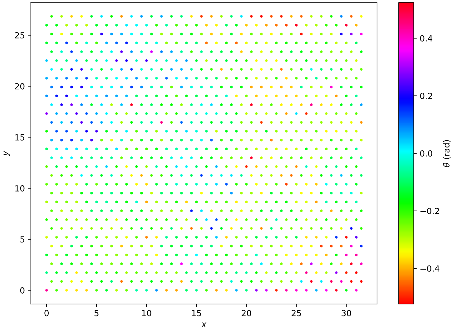
Hexagonal Lattice L=32 , T = 1.85e - 01
