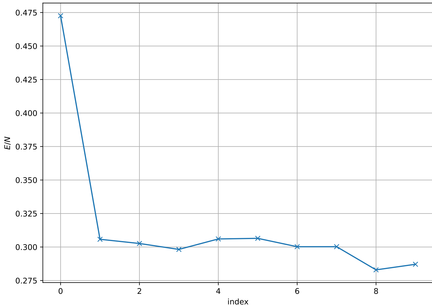
Energy per Site at T = 1.900e - 01 , L = 32
