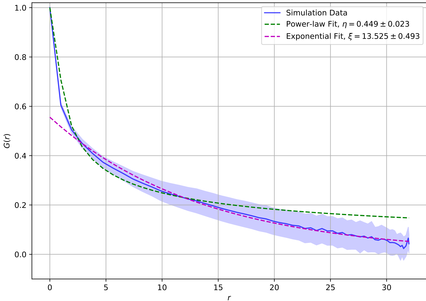
Correlation Function at T = 1.95e - 01 , L = 32
