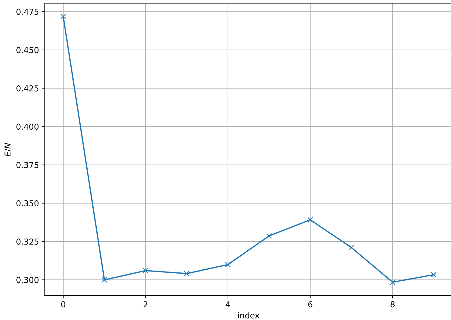
Energy per Site at T = 1.950e - 01 , L = 32
