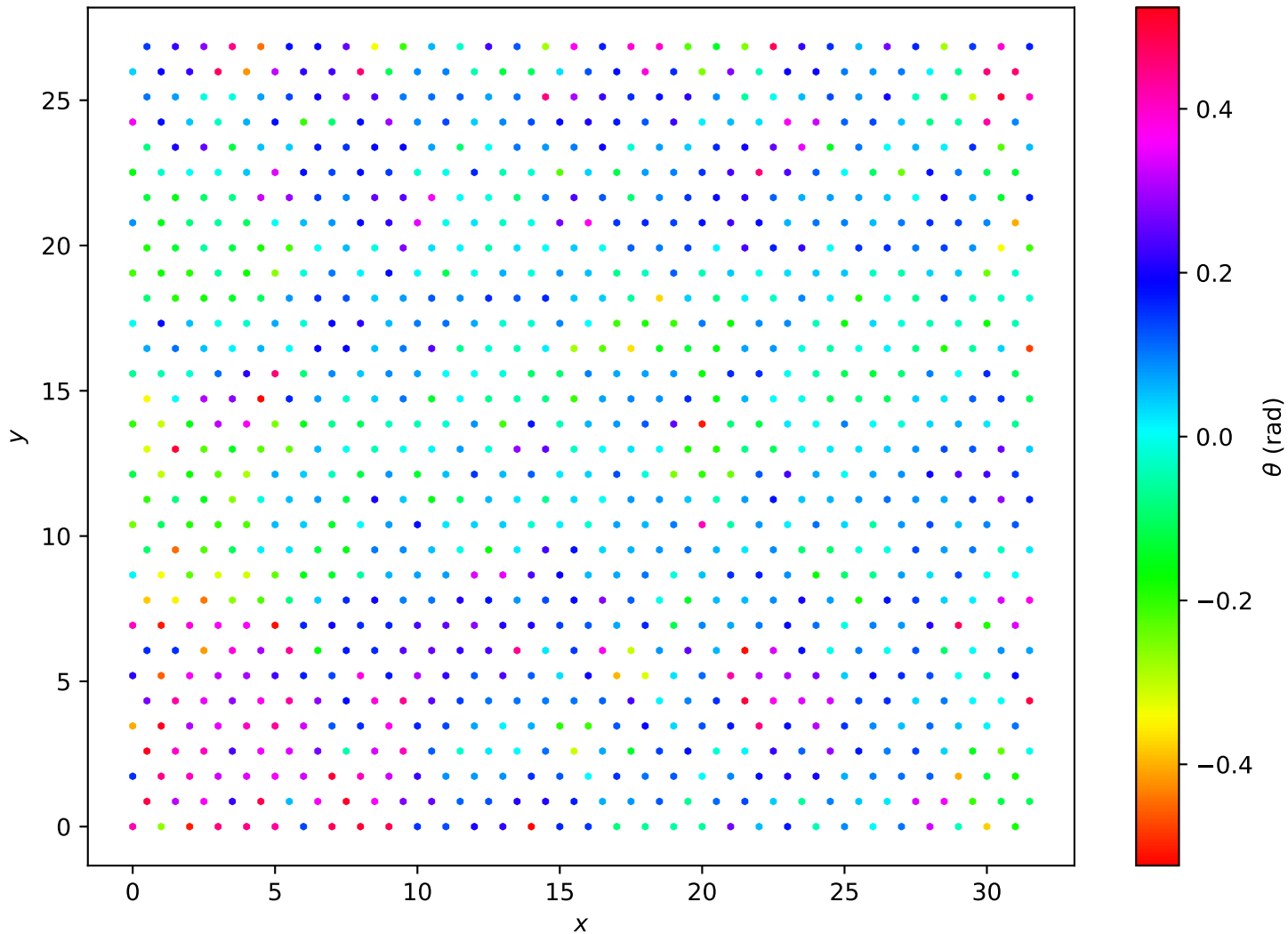
Hexagonal Lattice L=32 , T = 1.95e - 01
