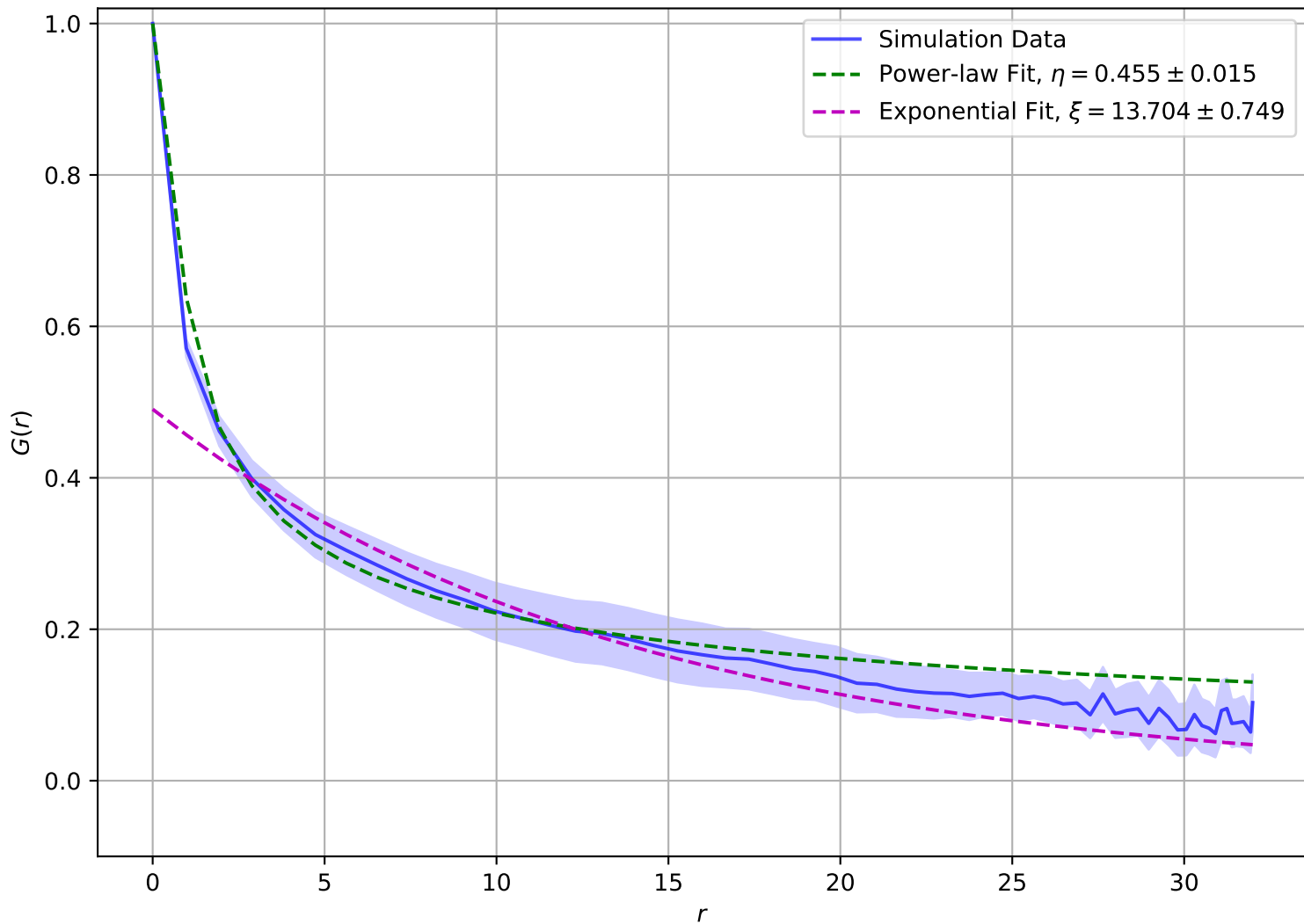
Correlation Function at T = 2.00e - 01 , L = 32
