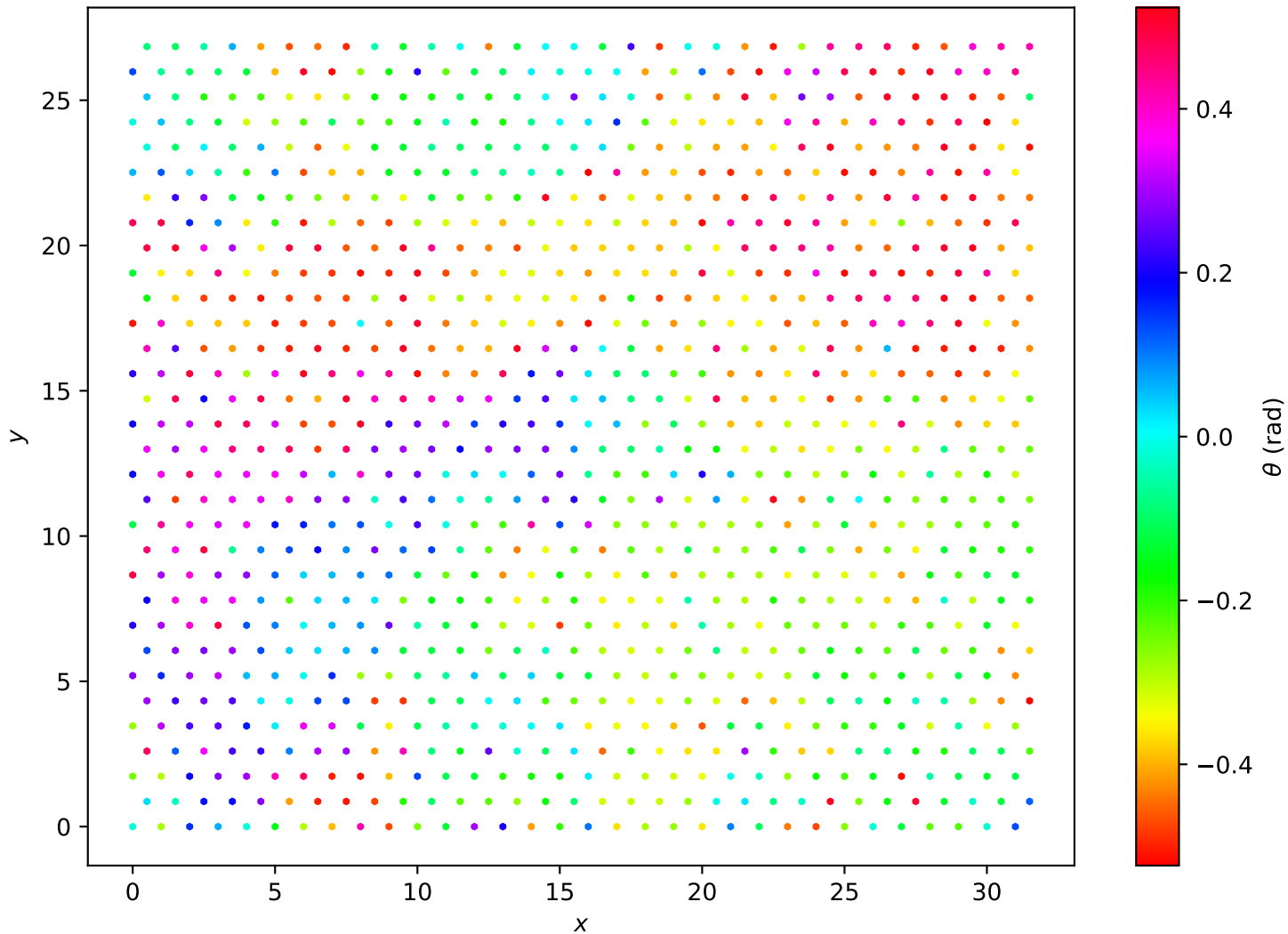
Hexagonal Lattice L=32 , T = 2.00e - 01
