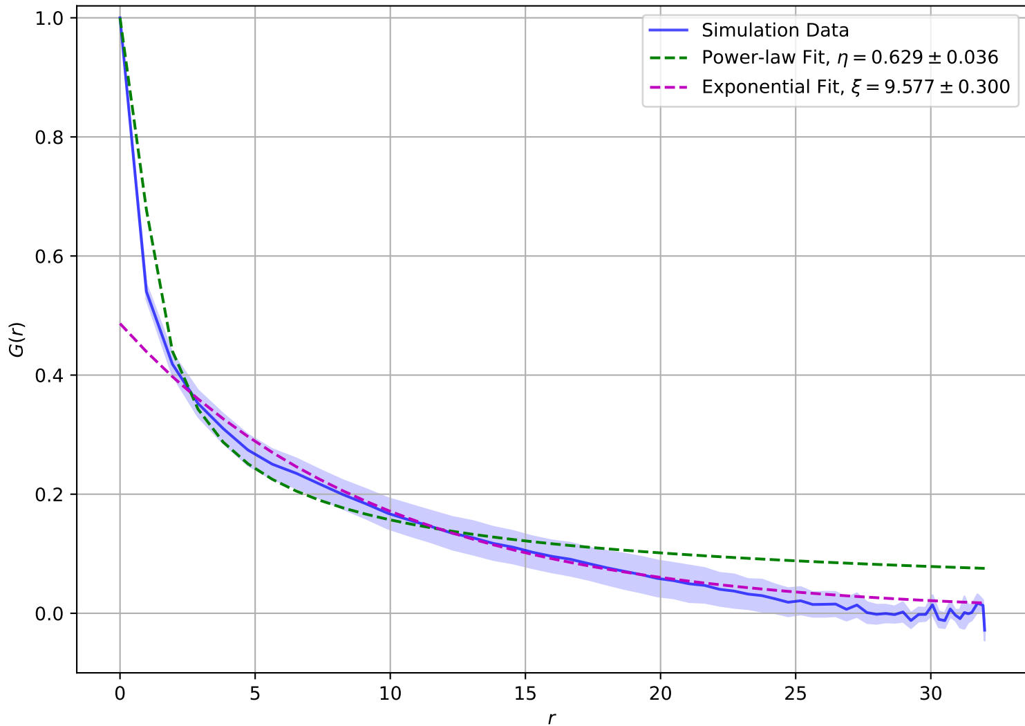
Correlation Function at T = 2.05e - 01 , L = 32
