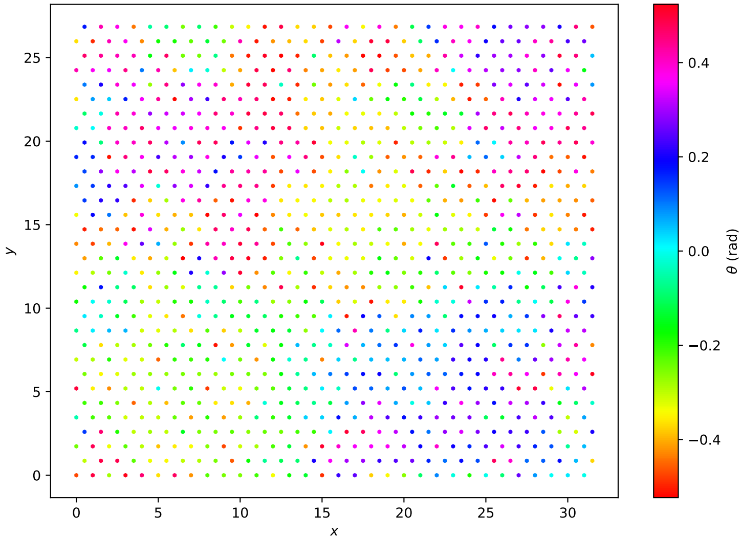
Hexagonal Lattice L=32 , T = 2.05e - 01
