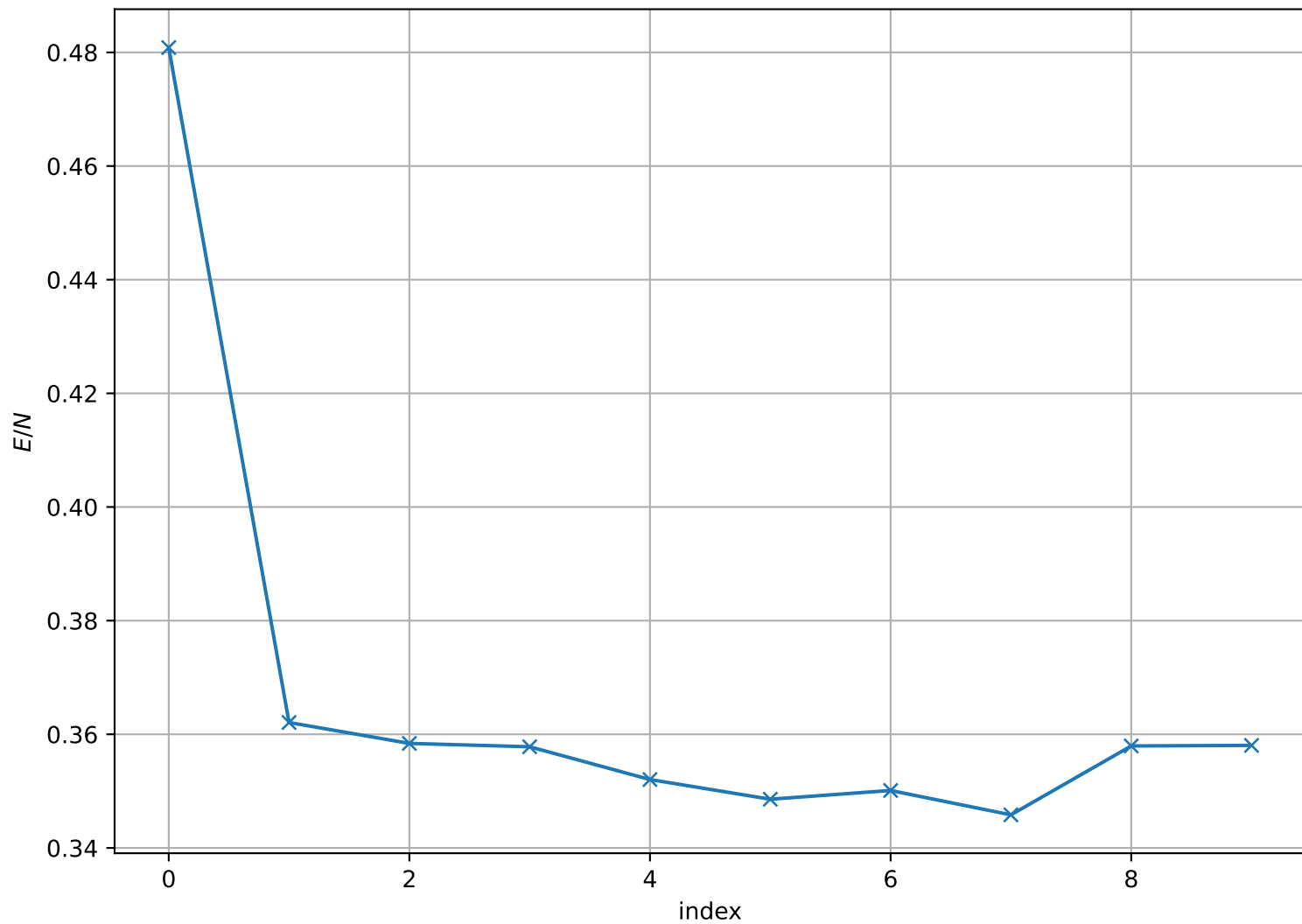
Energy per Site at T = 2.100e - 01 , L = 32
