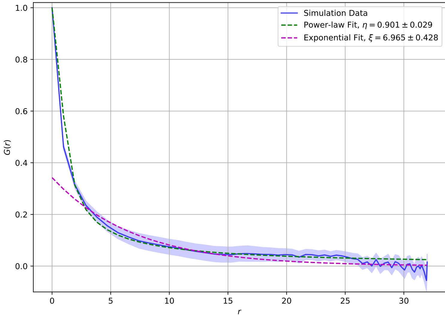
Correlation Function at T = 2.15e - 01 , L = 32
