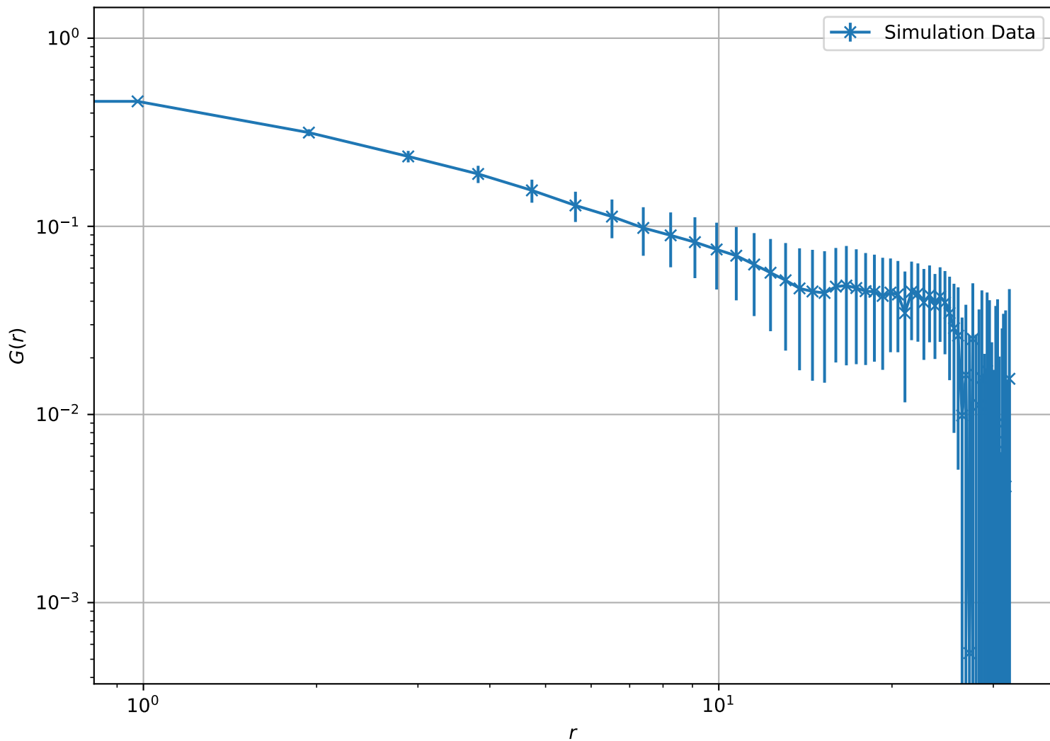
Correlation Function at T = 2.15e - 01 , L = 32 (Log-Log Scale)
