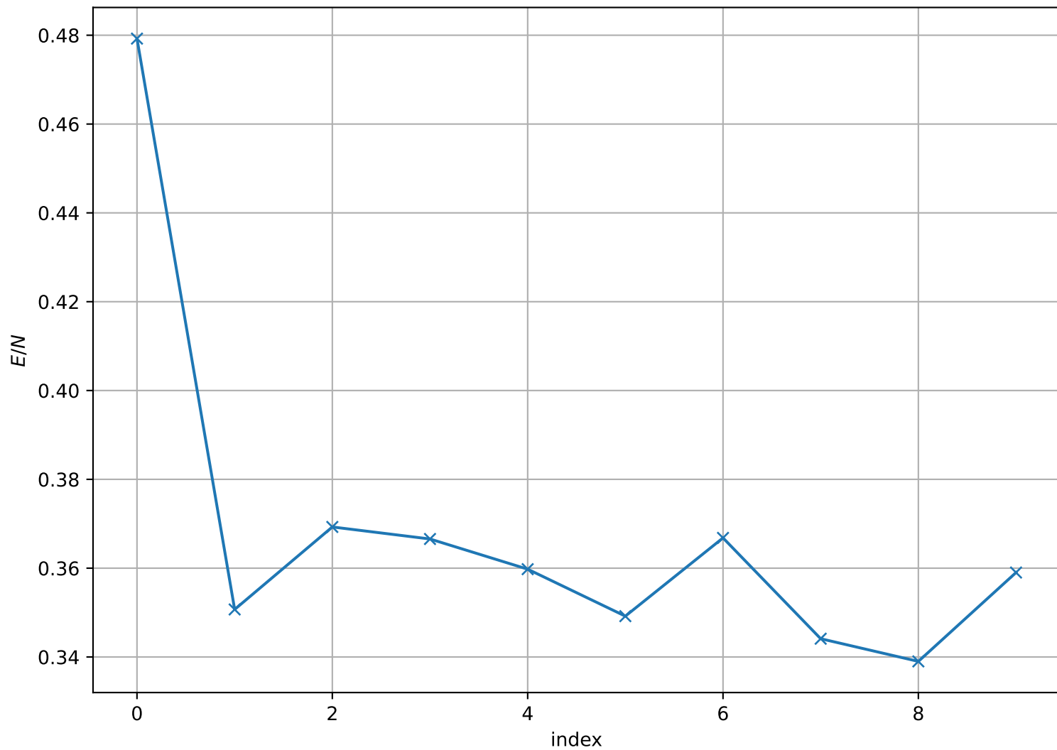
Energy per Site at T = 2.150e - 01 , L = 32
