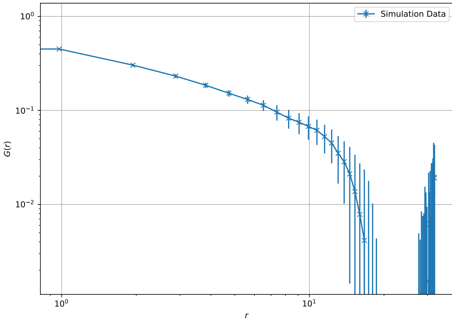
Correlation Function at T = 2.20e - 01 , L = 32 (Log-Log Scale)
