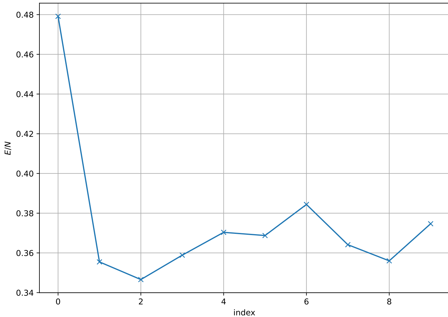
Energy per Site at T = 2.200e - 01 , L = 32
