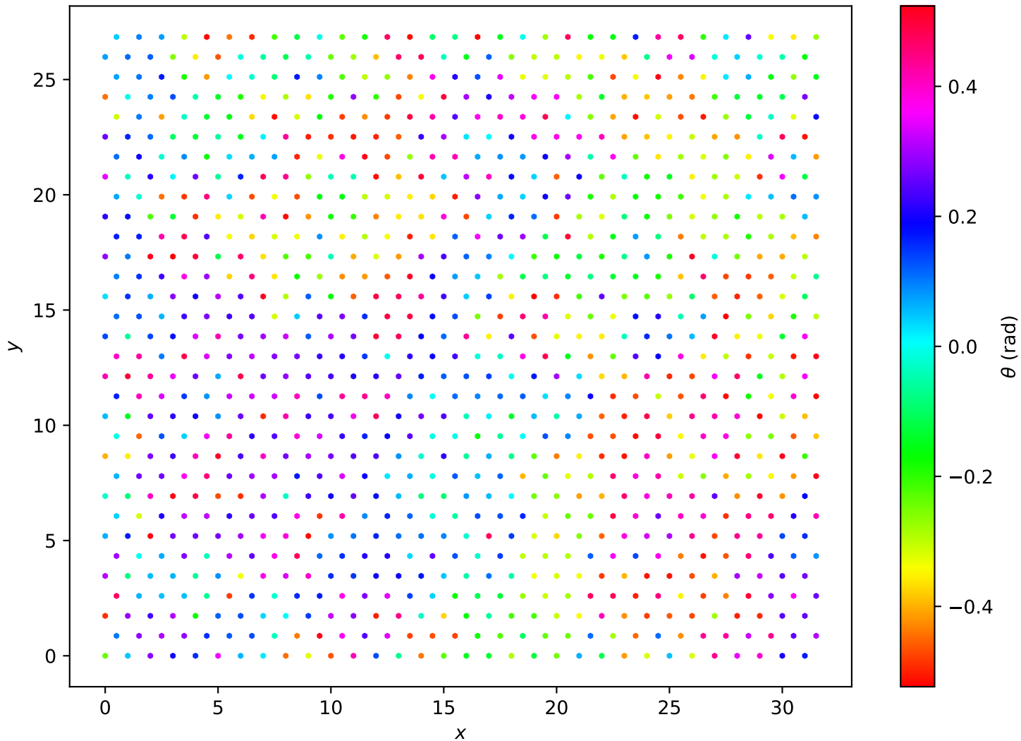
Hexagonal Lattice L=32 , T = 2.20e - 01
