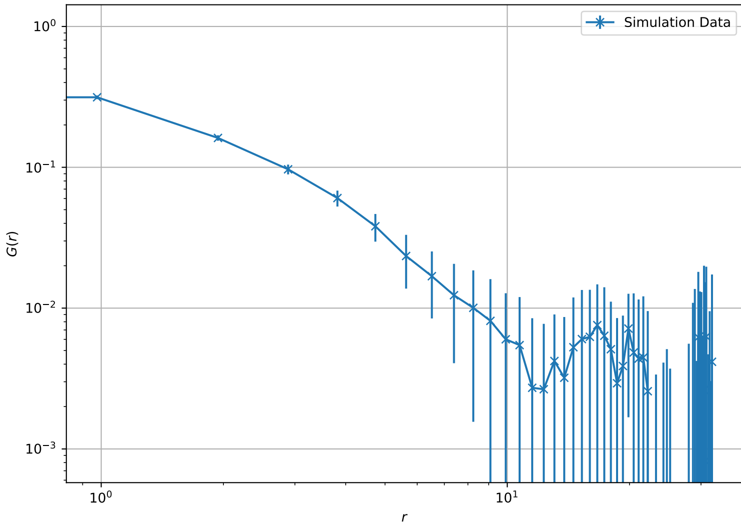
Correlation Function at T = 2.50e - 01 , L = 32 (Log-Log Scale)
