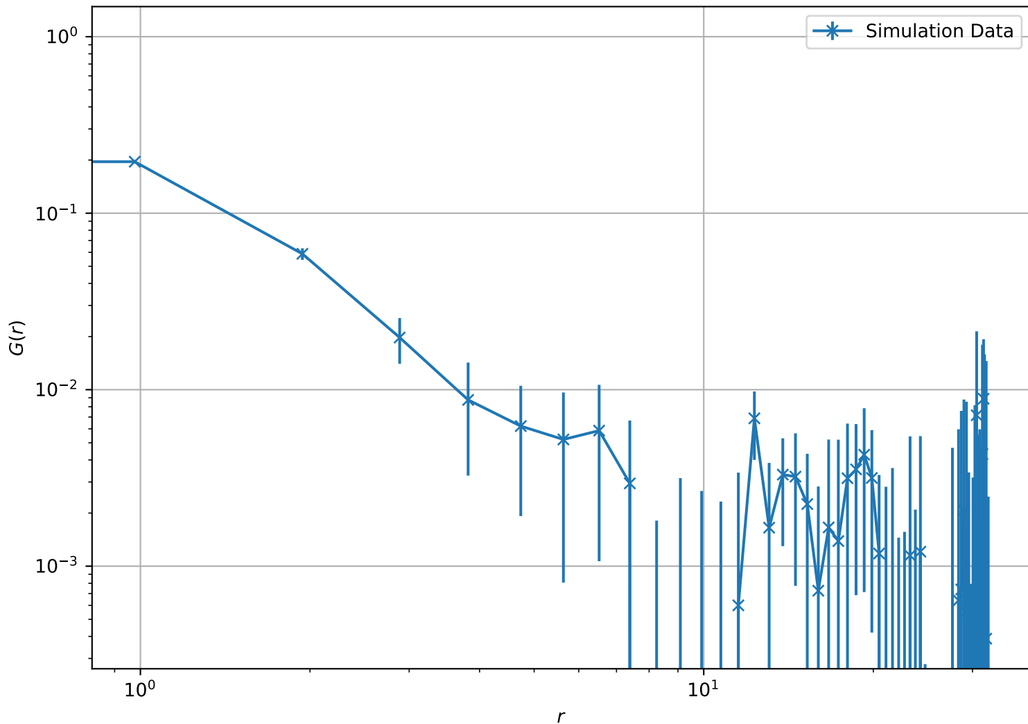
Correlation Function at T = 3.00e - 01 , L = 32 (Log-Log Scale)
