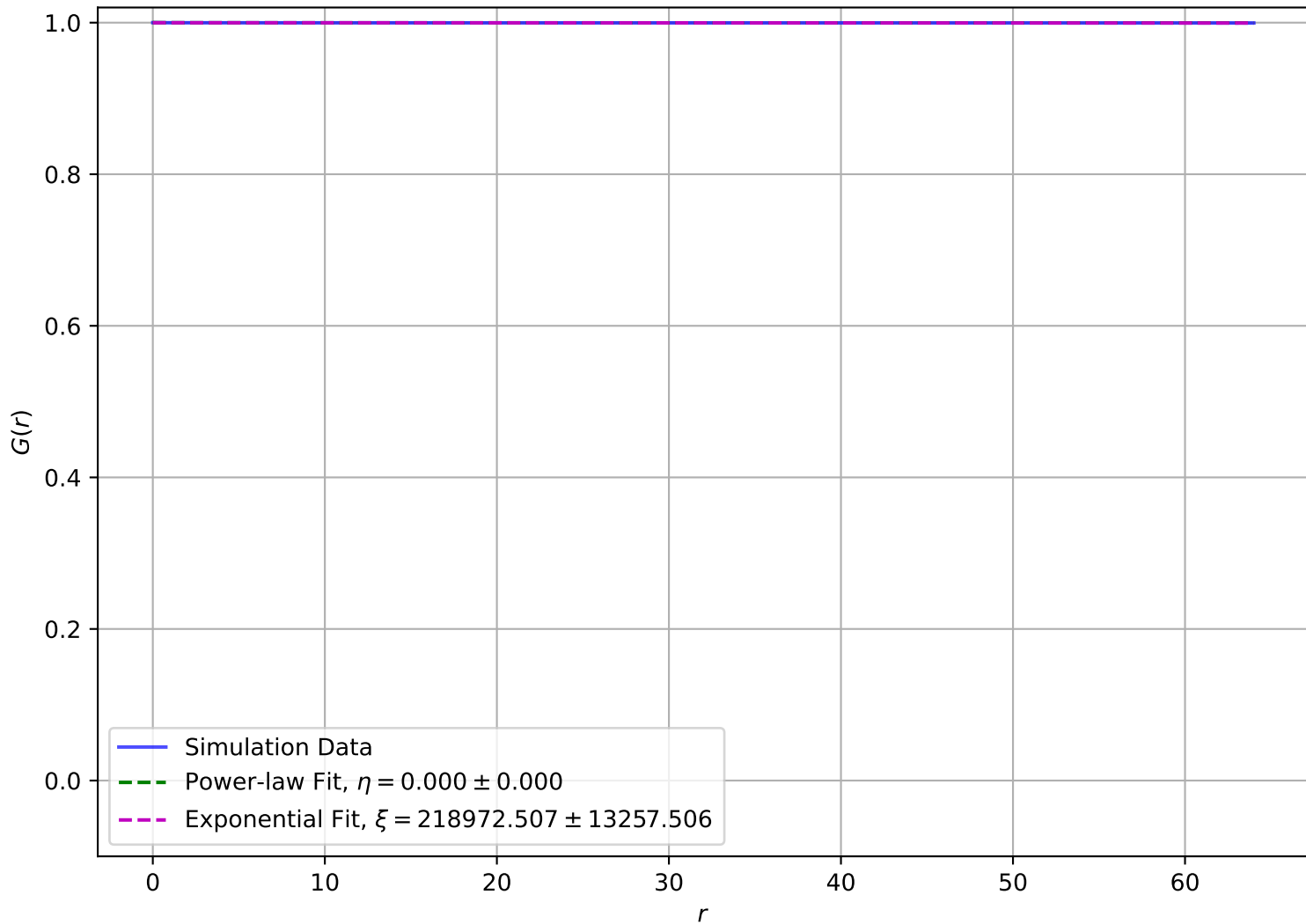
Correlation Function at T = 1.00\text{e} - 02 , L = 64
