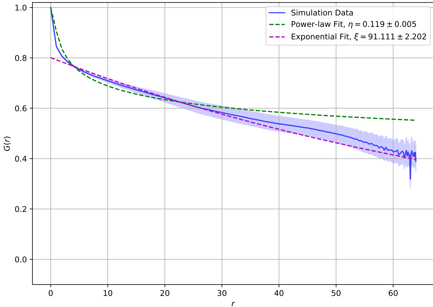
Correlation Function at T = 1.50e - 01 , L = 64
