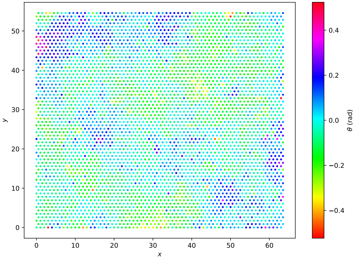
Hexagonal Lattice L=64 , T = 1.50e - 01
