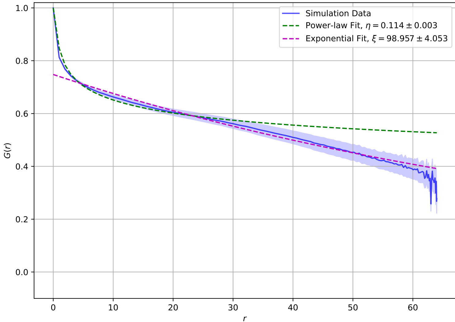
Correlation Function at T = 1.60e - 01 , L = 64
