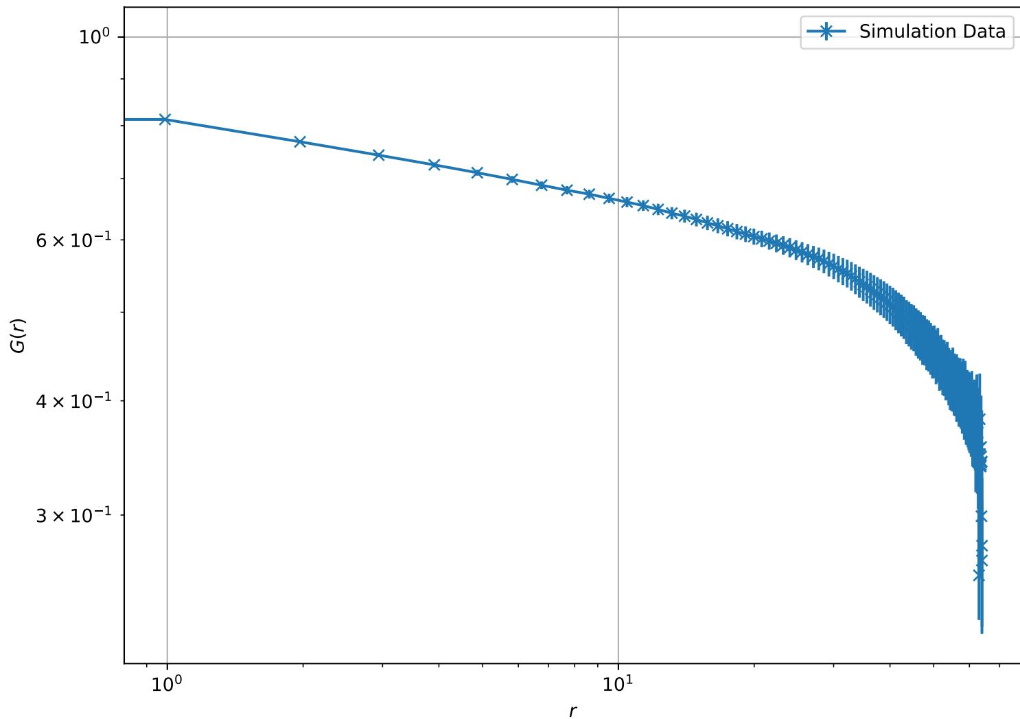
Correlation Function at T = 1.60e - 01 , L = 64 (Log-Log Scale)
