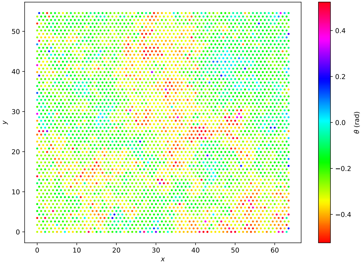
Hexagonal Lattice L=64 , T = 1.60e - 01
