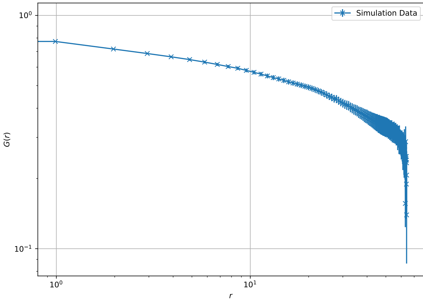
Correlation Function at T = 1.70e - 01 , L = 64 (Log-Log Scale)
