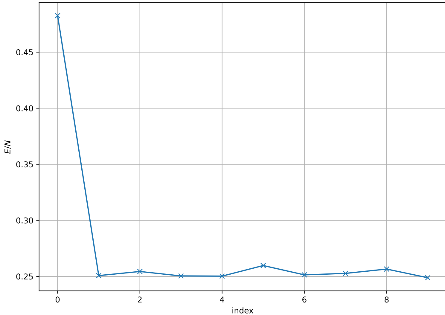
Energy per Site at T = 1.700e - 01 , L = 64
