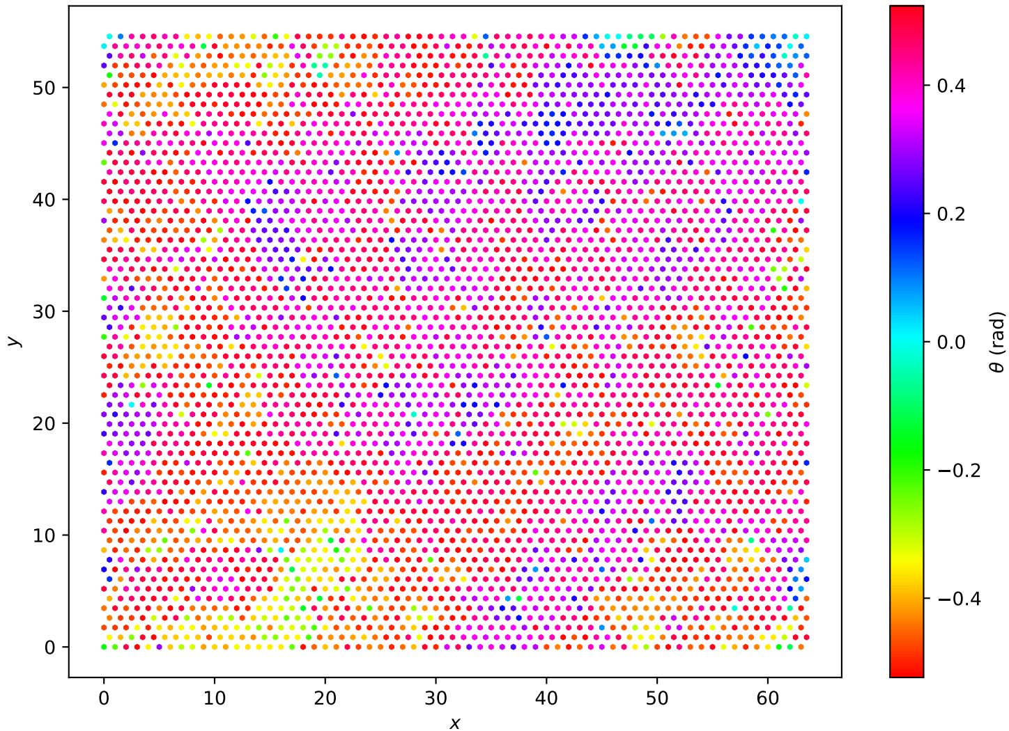
Hexagonal Lattice L=64 , T = 1.70e - 01
