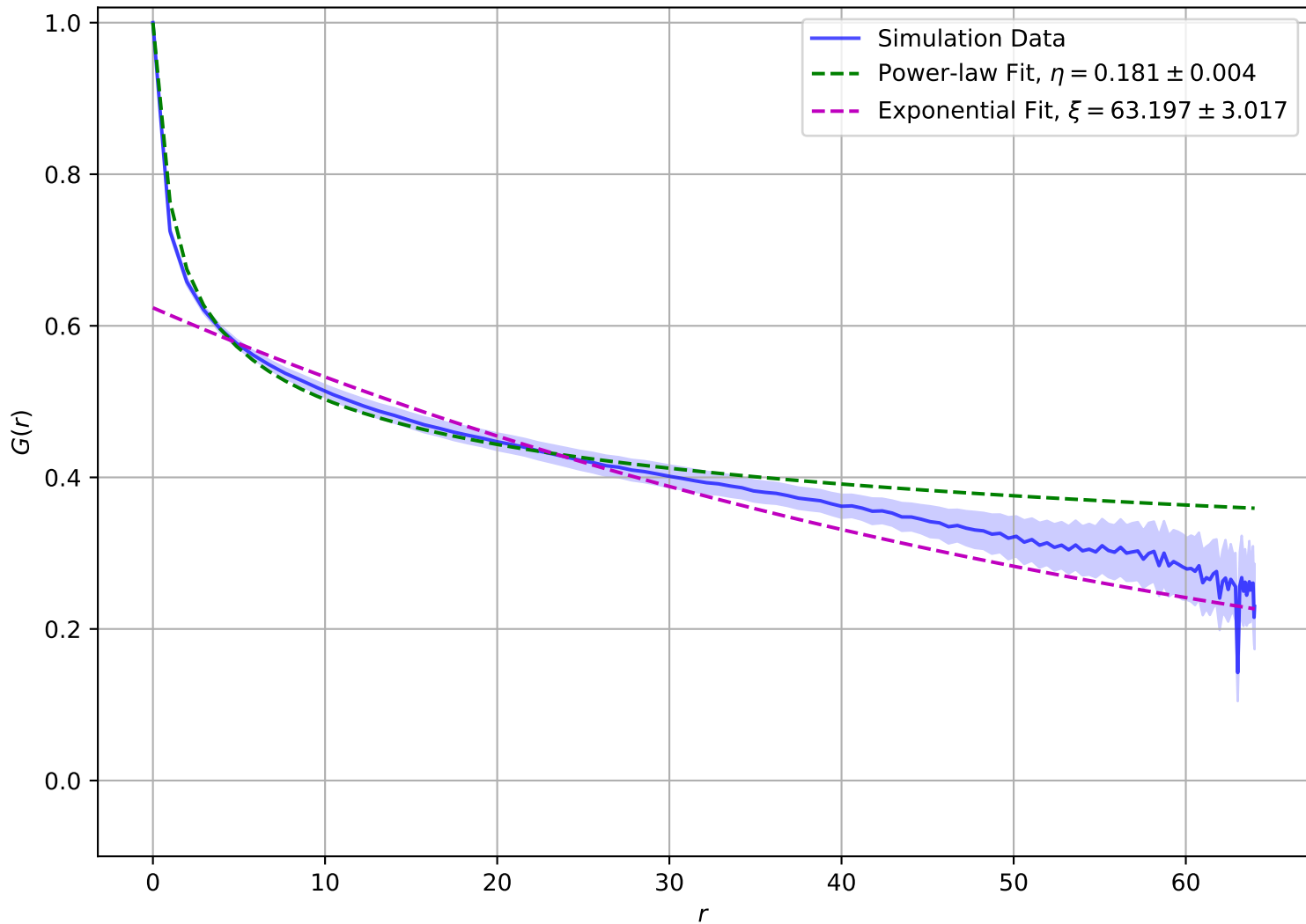
Correlation Function at T = 1.80e - 01 , L = 64
