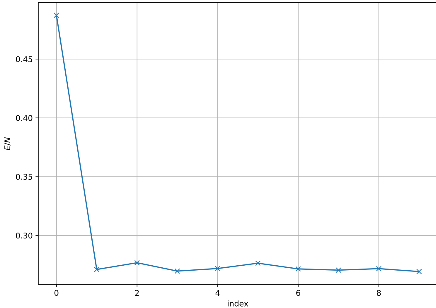
Energy per Site at T = 1.800e - 01 , L = 64
