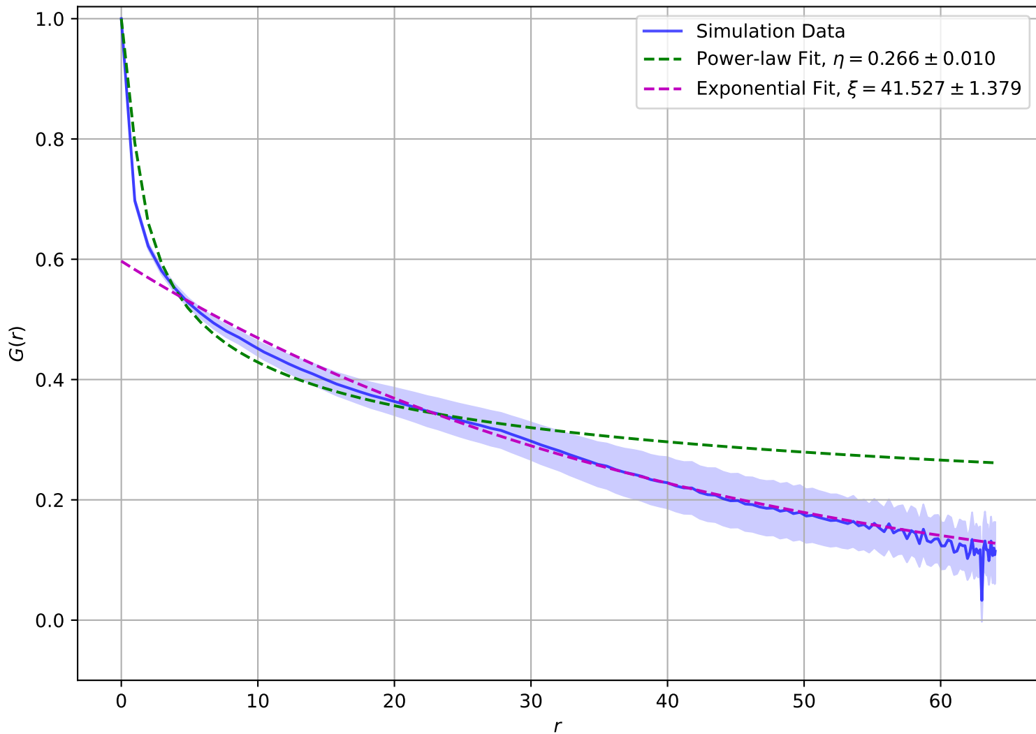
Correlation Function at T = 1.85e - 01 , L = 64
