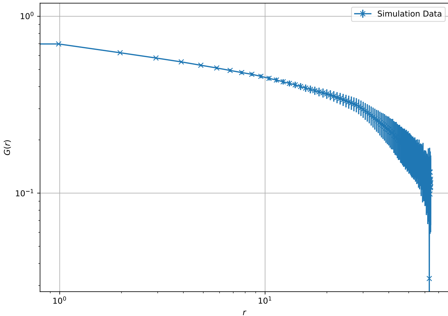
Correlation Function at T = 1.85e - 01 , L = 64 (Log-Log Scale)
