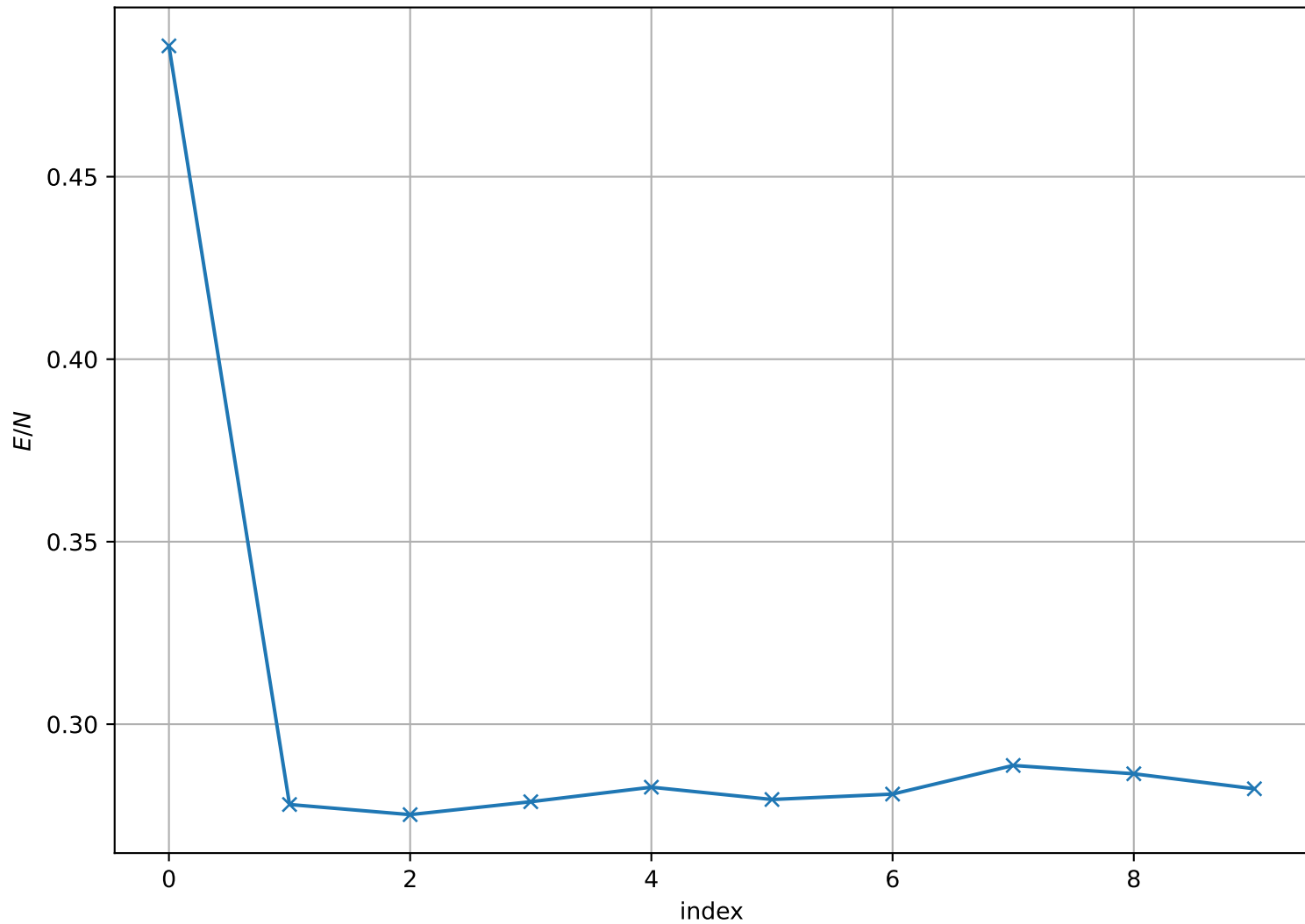
Energy per Site at T = 1.850e - 01 , L = 64
