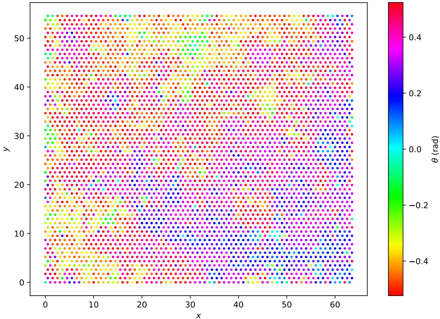
Hexagonal Lattice L=64 , T = 1.85e - 01
