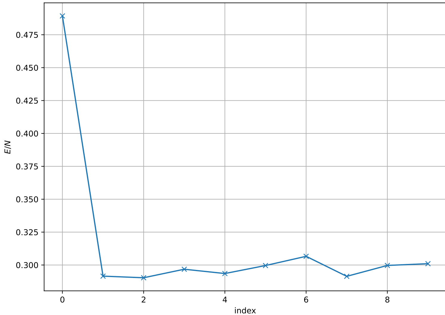
Energy per Site at T = 1.900e - 01 , L = 64
