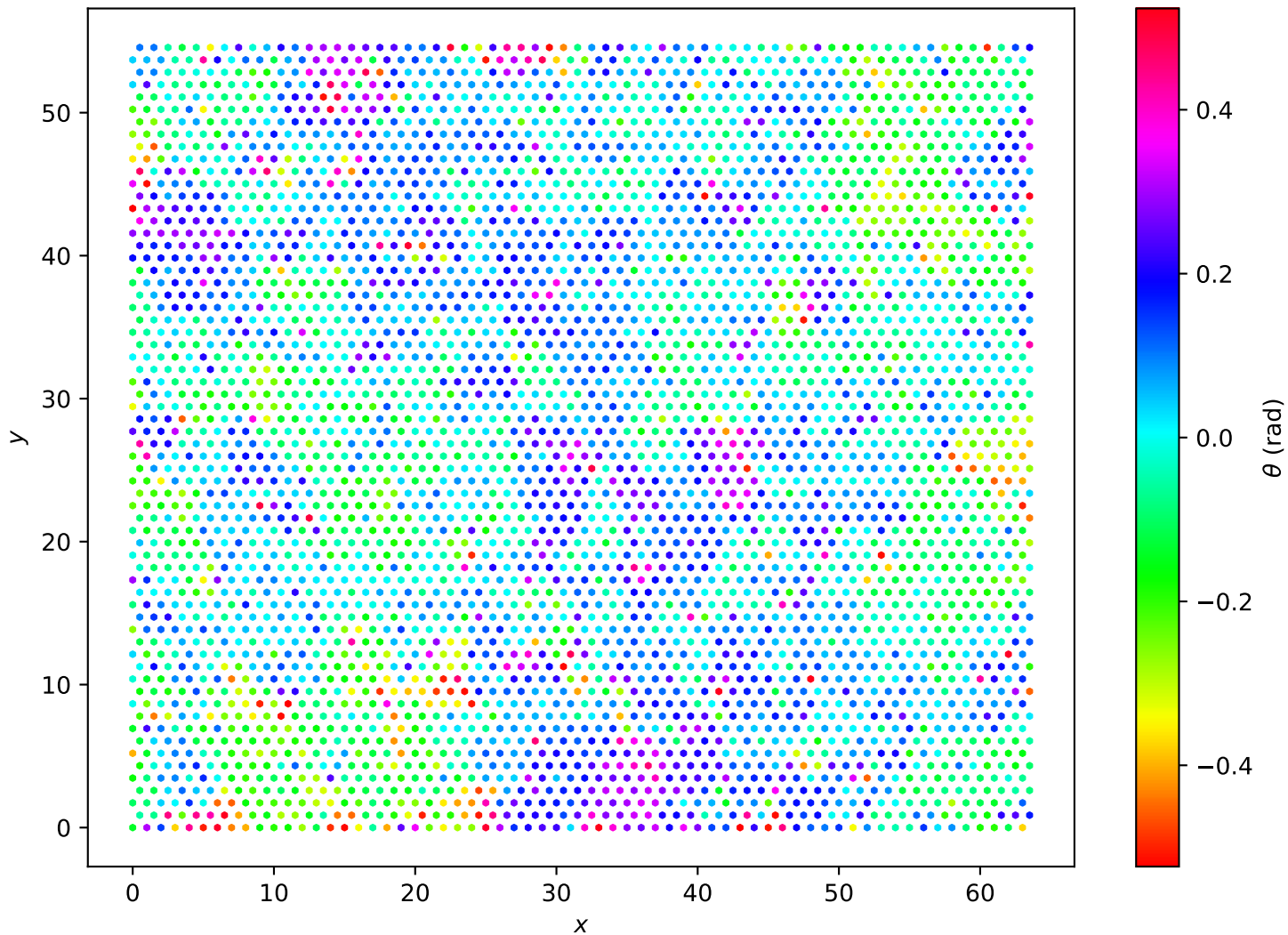
Hexagonal Lattice L=64 , T = 1.90e - 01
