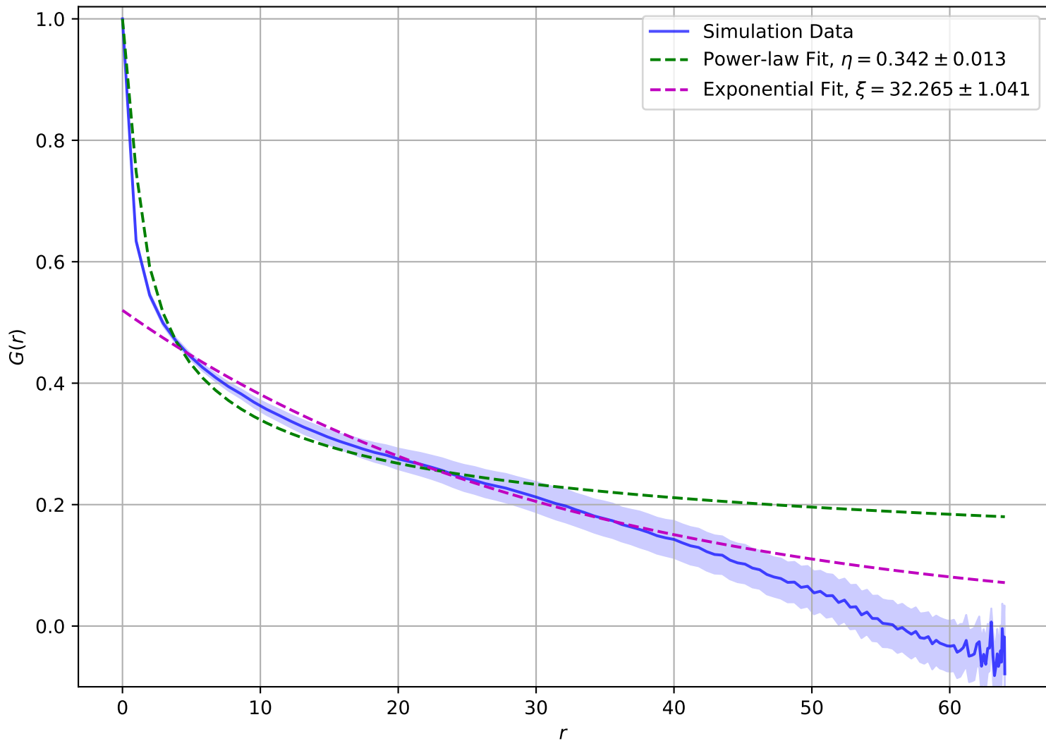
Correlation Function at T = 1.95e - 01 , L = 64
