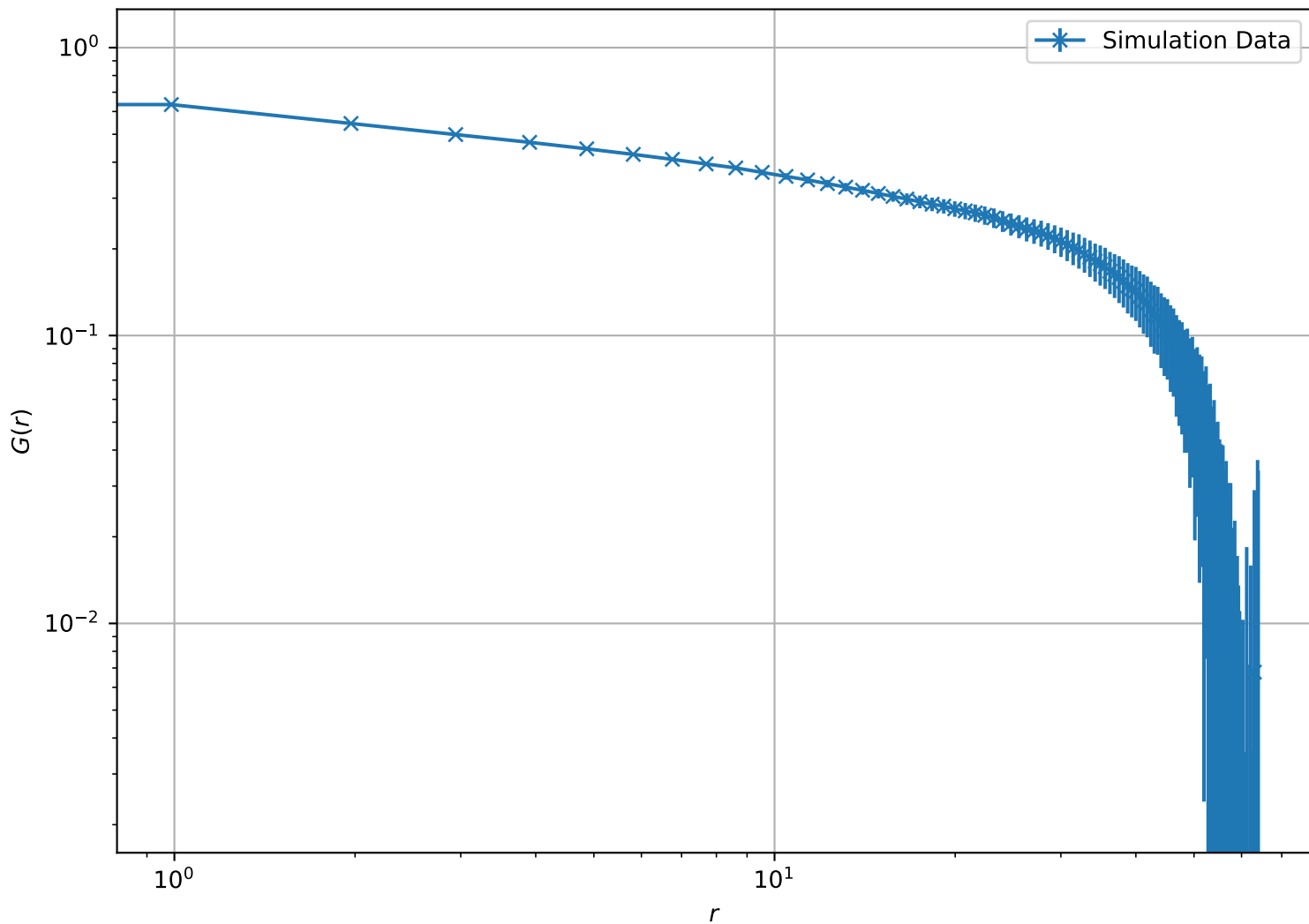
Correlation Function at T = 1.95e - 01 , L = 64 (Log-Log Scale)
