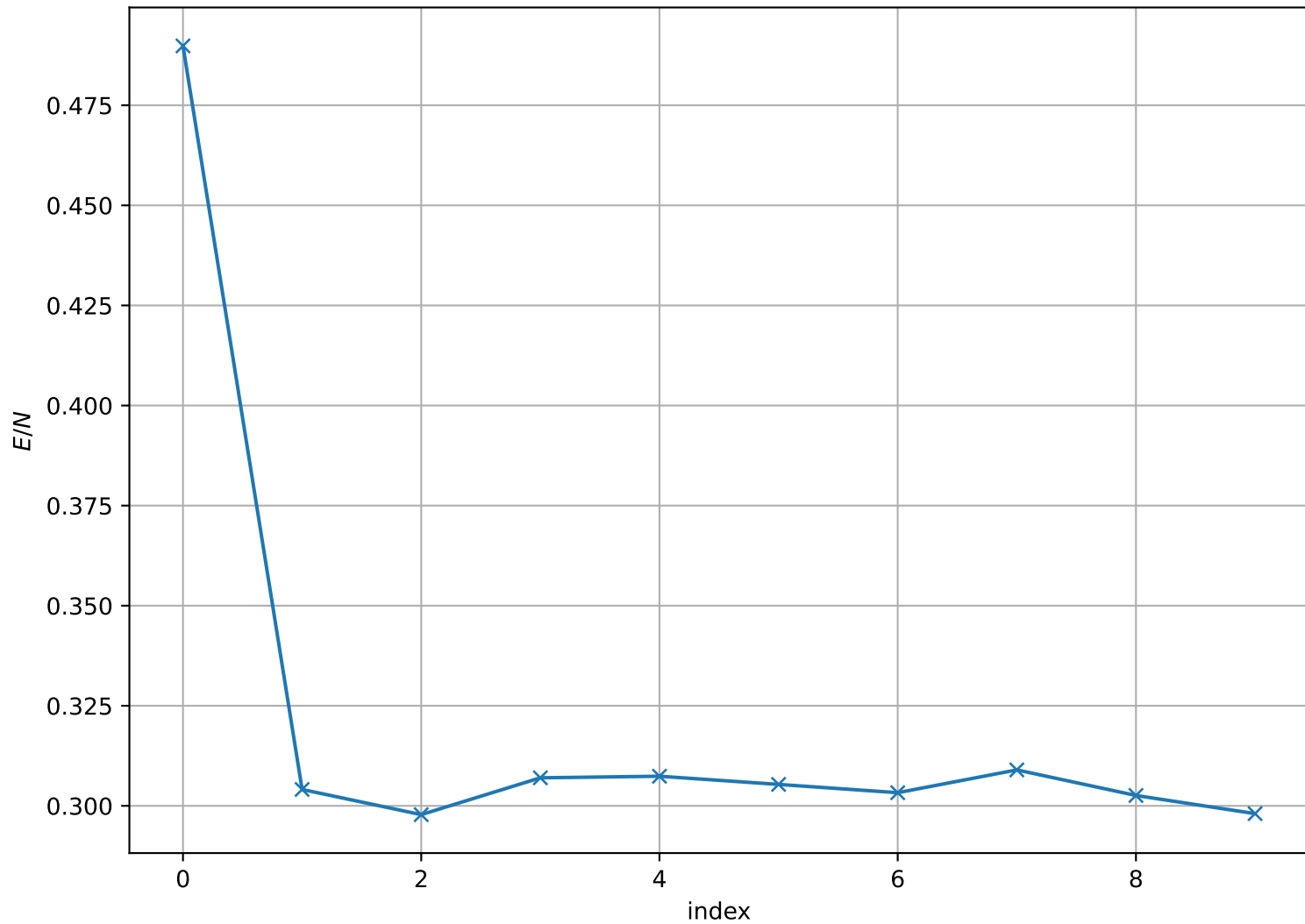
Energy per Site at T = 1.950e - 01 , L = 64
