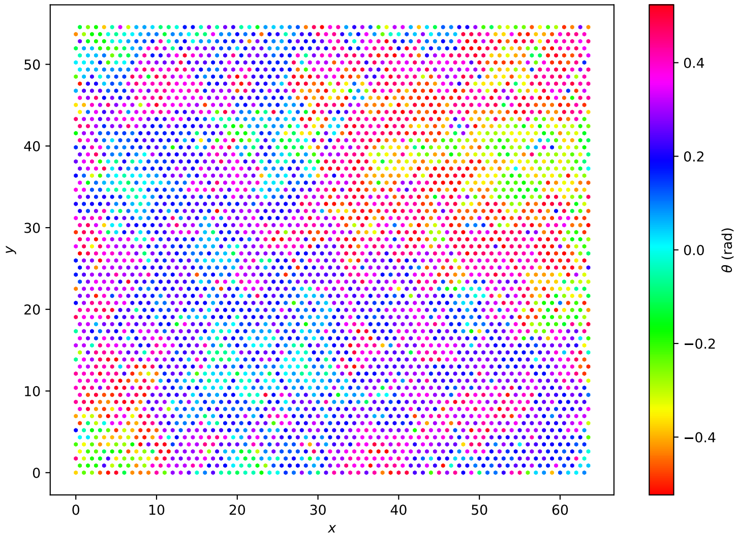
Hexagonal Lattice L=64 , T = 1.95e - 01
