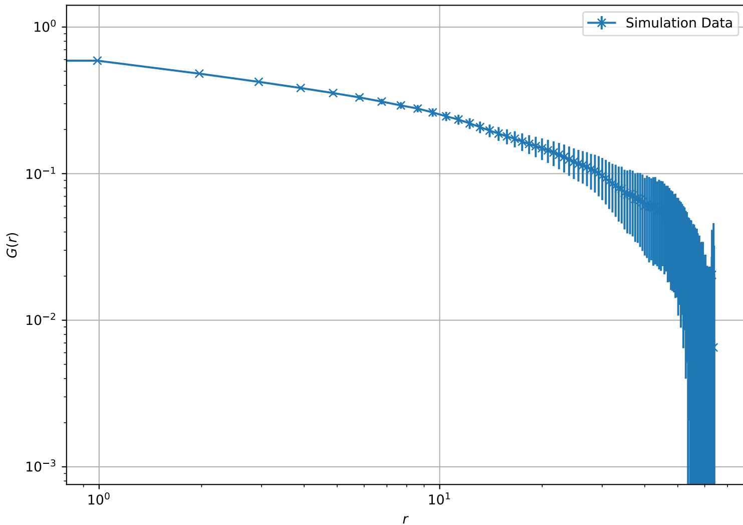
Correlation Function at T = 2.00e - 01 , L = 64 (Log-Log Scale)
