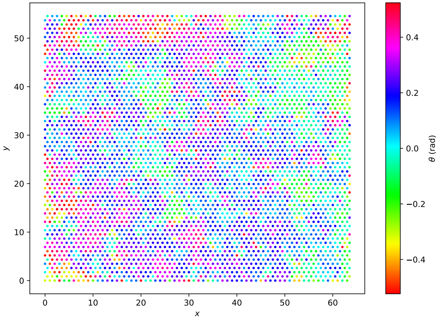
Hexagonal Lattice L=64 , T = 2.00e - 01
