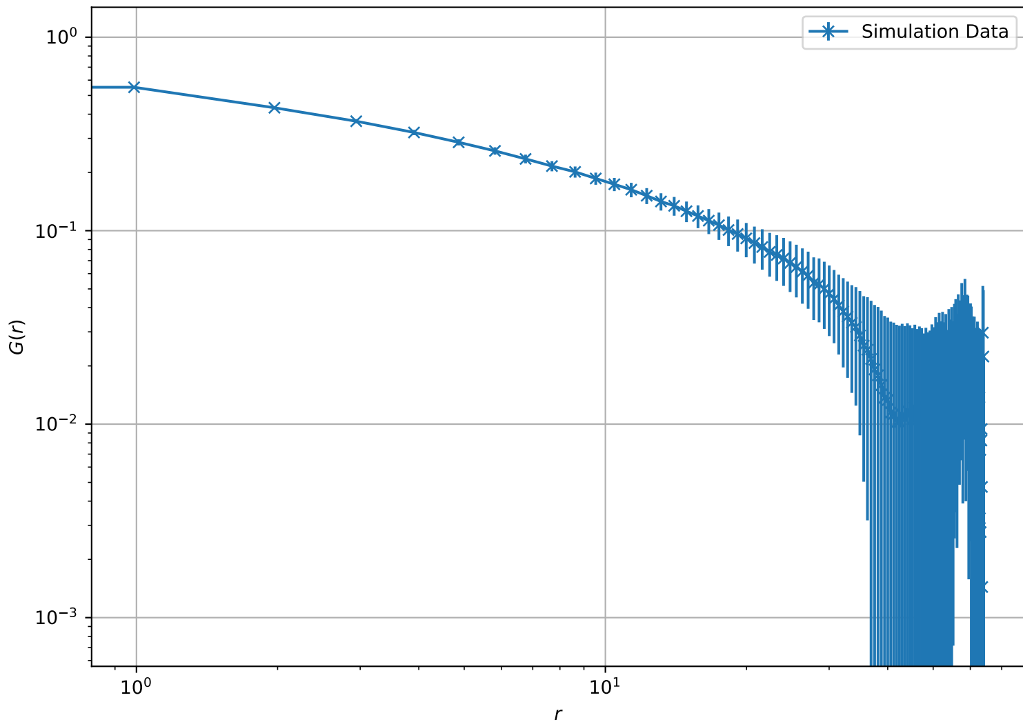
Correlation Function at T = 2.05e - 01 , L = 64 (Log-Log Scale)
