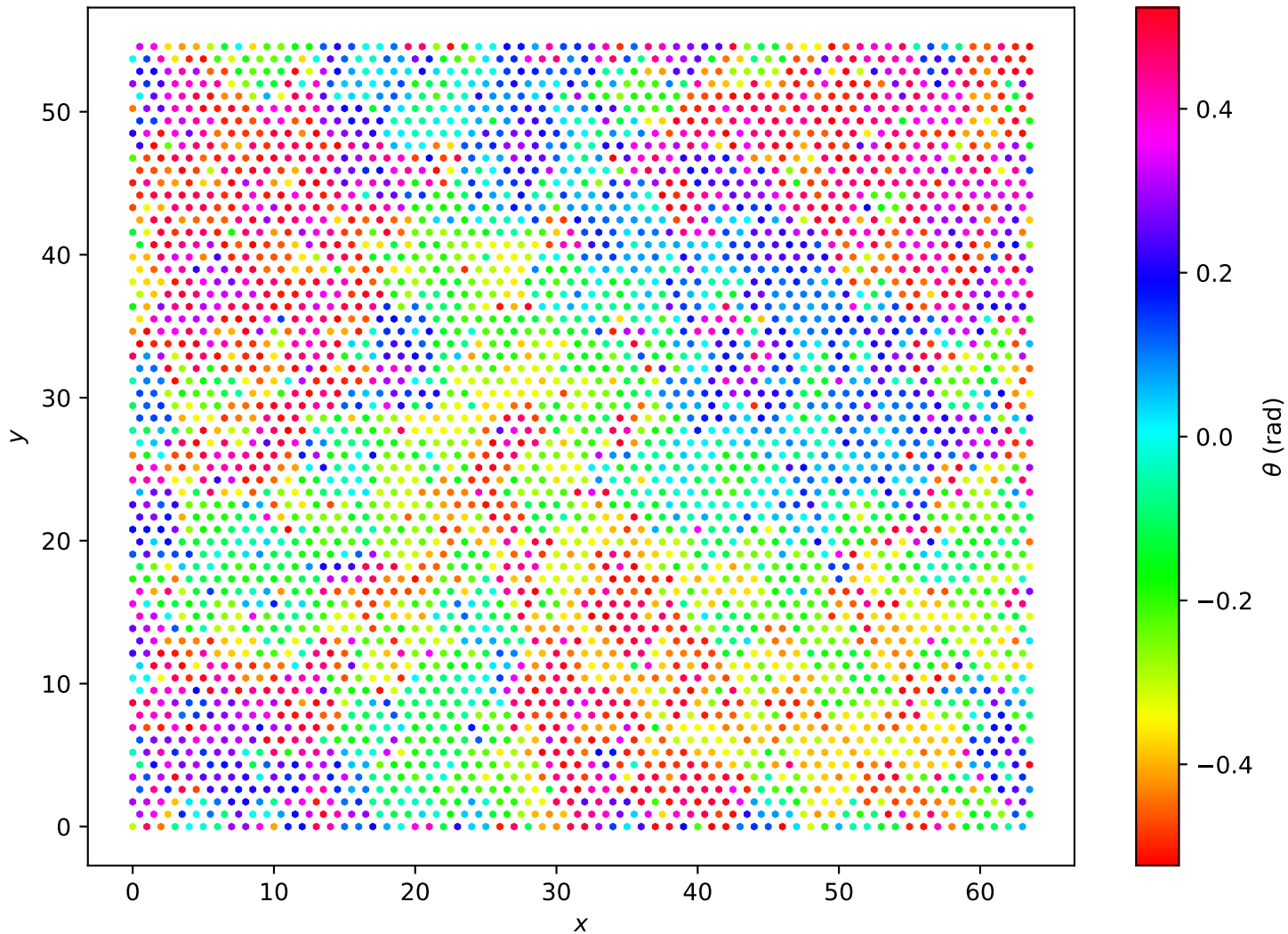
Hexagonal Lattice L=64 , T = 2.05e - 01
