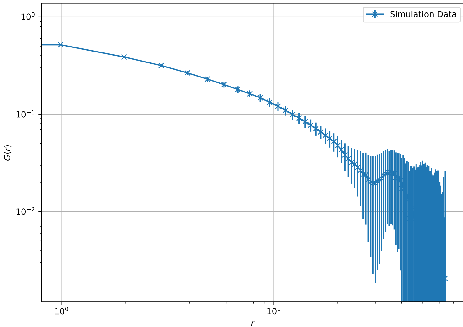
Correlation Function at T = 2.10e - 01 , L = 64 (Log-Log Scale)
