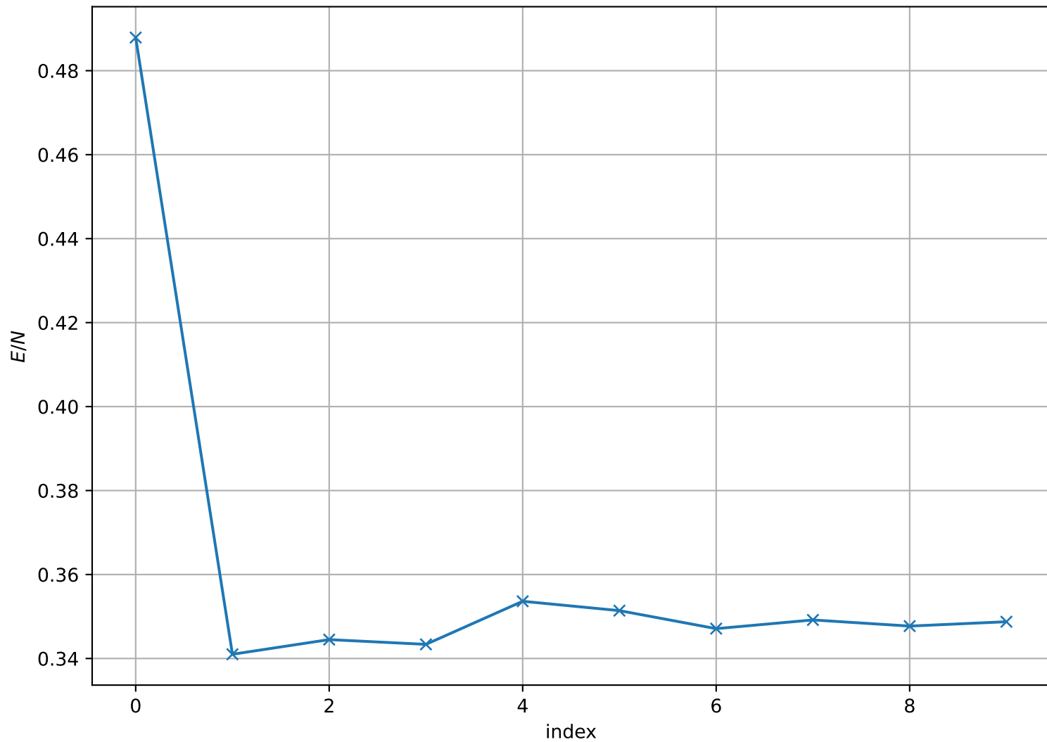
Energy per Site at T = 2.100e - 01 , L = 64
