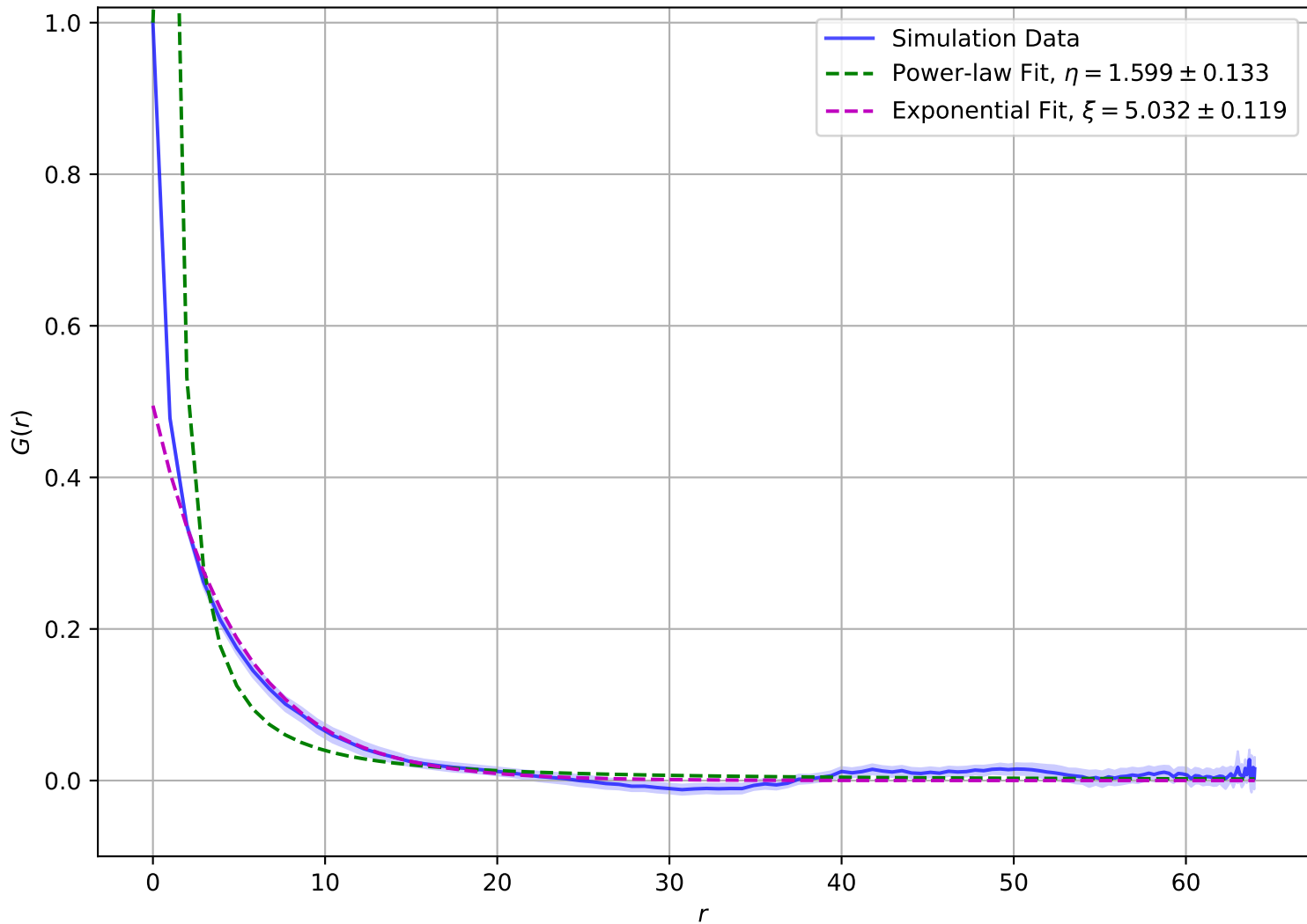
Correlation Function at T = 2.15e - 01 , L = 64
