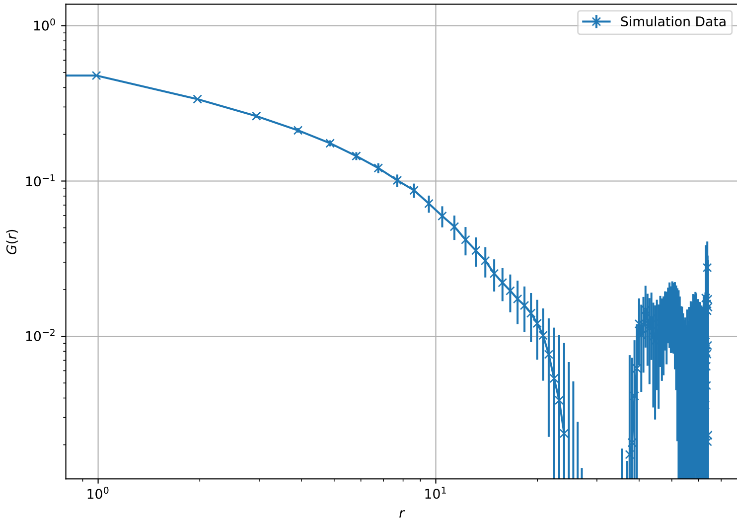
Correlation Function at T = 2.15e - 01 , L = 64 (Log-Log Scale)
